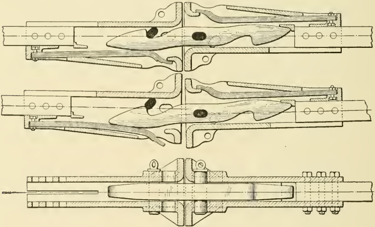
Fig. 120. Sectional Views of Link Coupler
